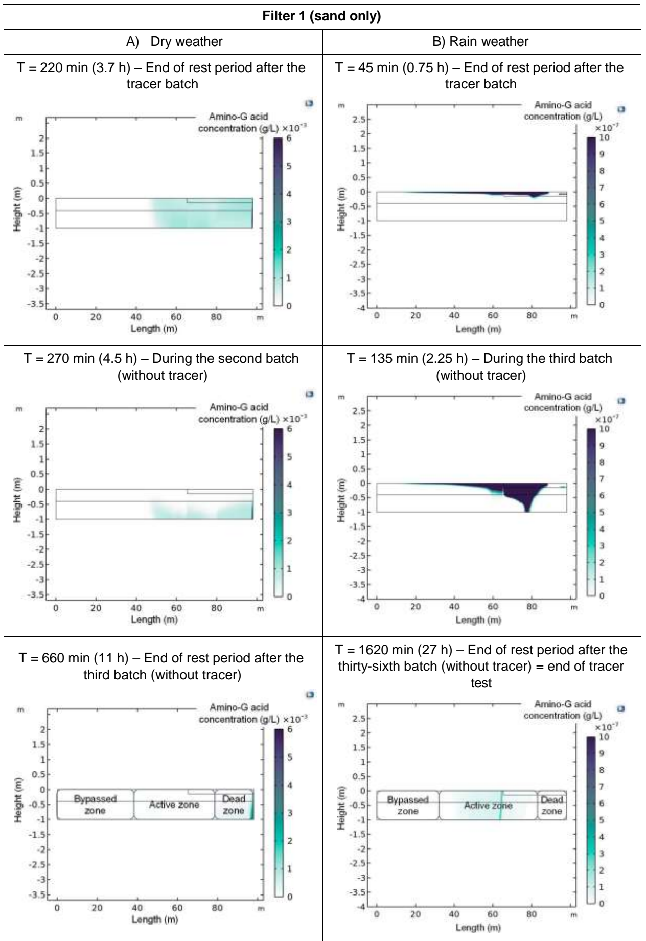
Figure 14: Evolution of the distribution of the amino-G acid concentration at different simulation times of the tracer test in filter 1 for 'dry weather' (A) and 'rain weather' (B) modes
